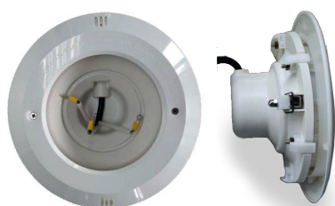
PROJECTOR HP-4602-72 EQUIVALENT TO PROJECTOR AP-07838 Lamp not included
